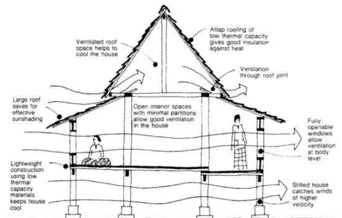
Illustration 1: Climate control in a traditional ASEAN house
