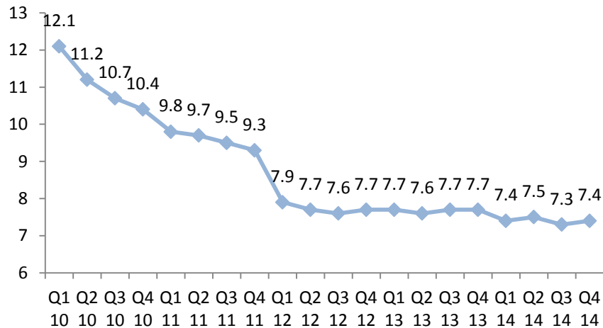
GDP Growth (%)
