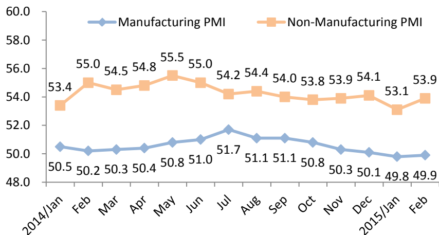
National PMI
