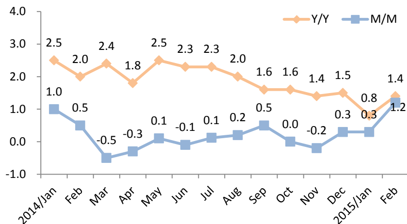
National PMI
